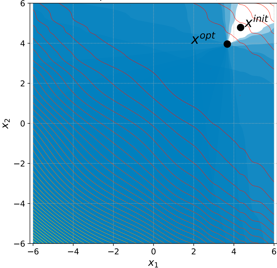
22 Rotated Ellipsoid with 6+n/2 constraints, instance=8
