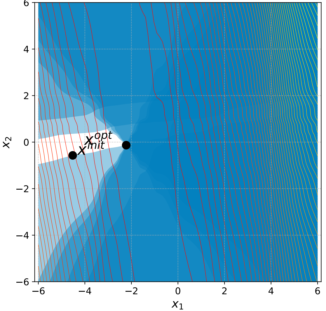
22 Rotated Ellipsoid with 6+n/2 constraints, instance=7
