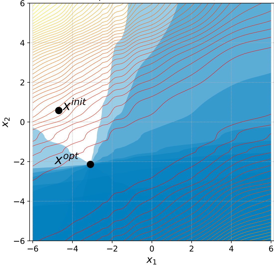
22 Rotated Ellipsoid with 6+n/2 constraints, instance=6
