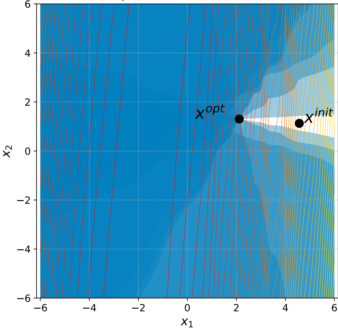
22 Rotated Ellipsoid with 6+n/2 constraints, instance=5
