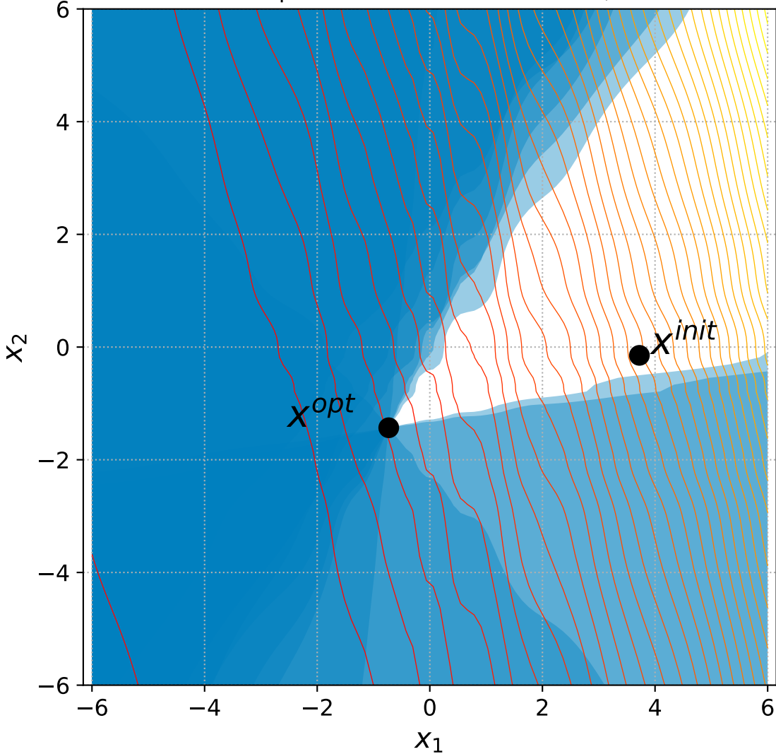
22 Rotated Ellipsoid with 6+n/2 constraints, instance=2
