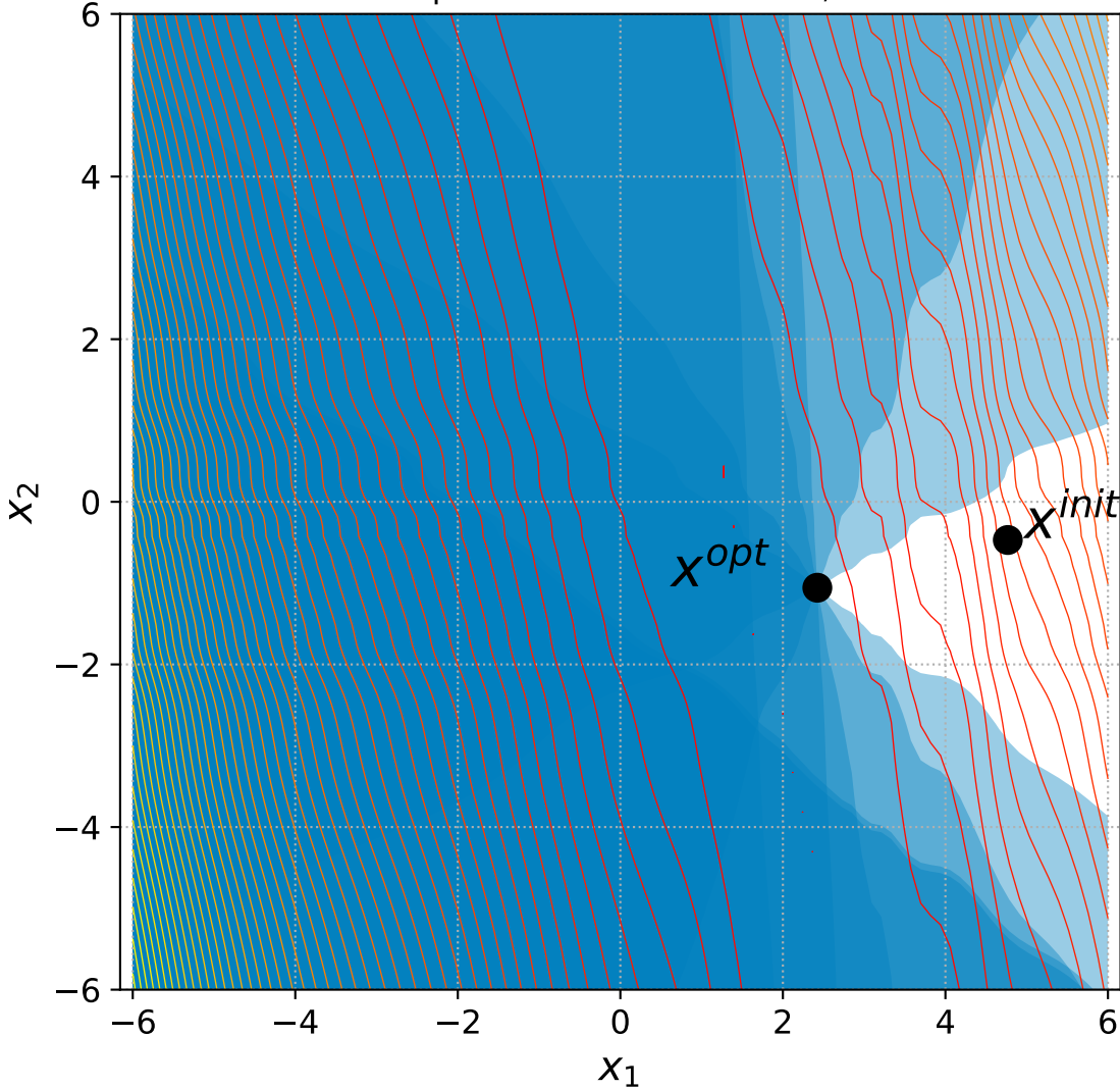
21 Rotated Ellipsoid with 6 constraints, instance=15
