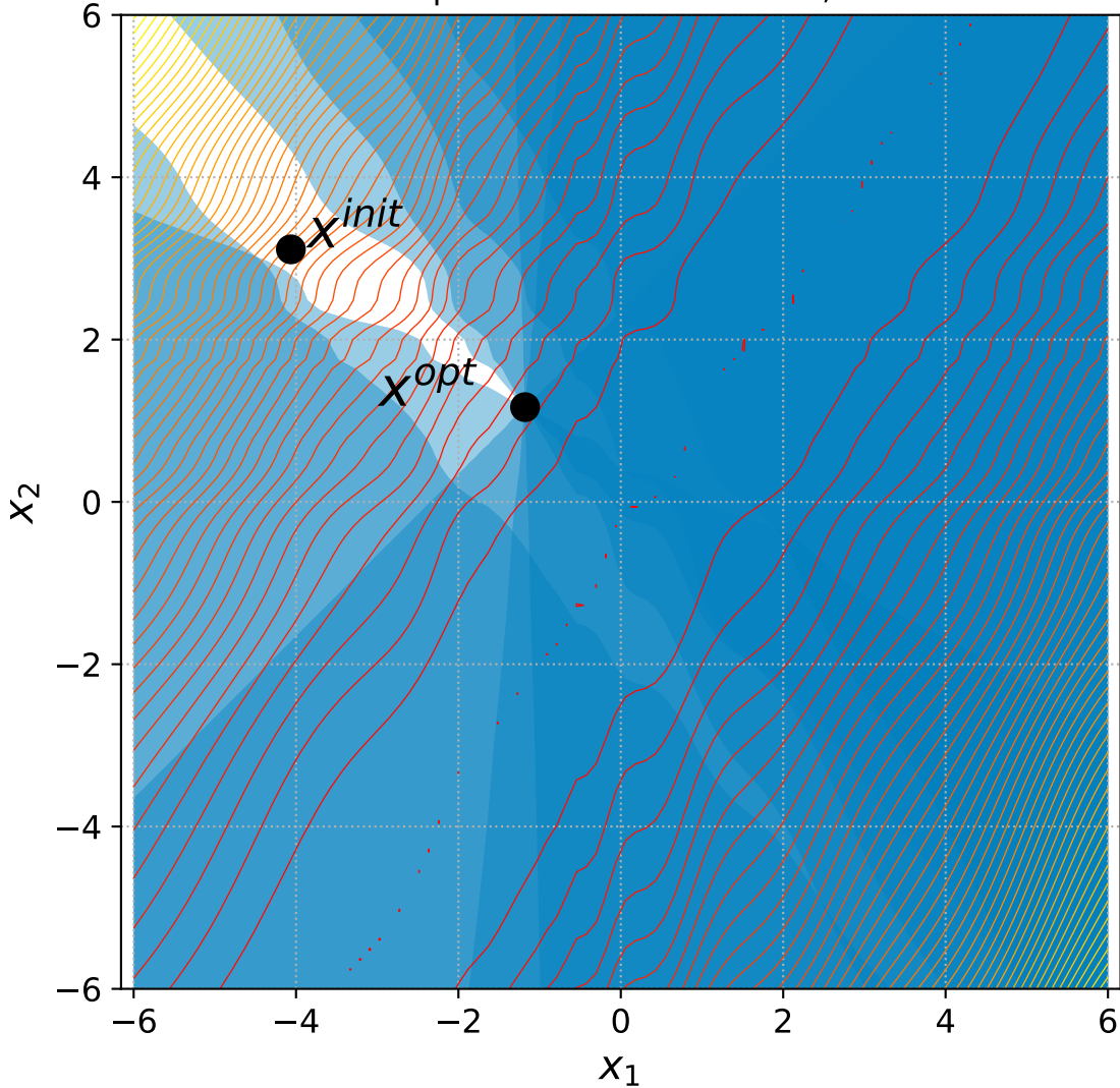
21 Rotated Ellipsoid with 6 constraints, instance=14
