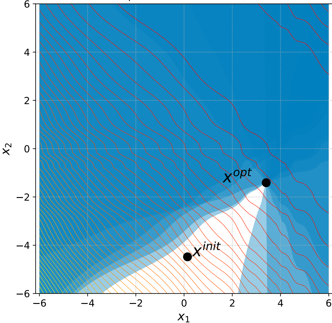
21 Rotated Ellipsoid with 6 constraints, instance=13
