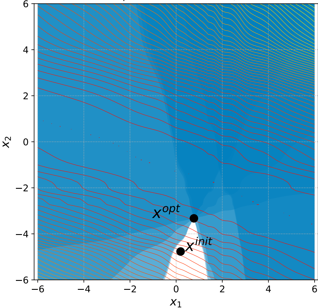
21 Rotated Ellipsoid with 6 constraints, instance=12
