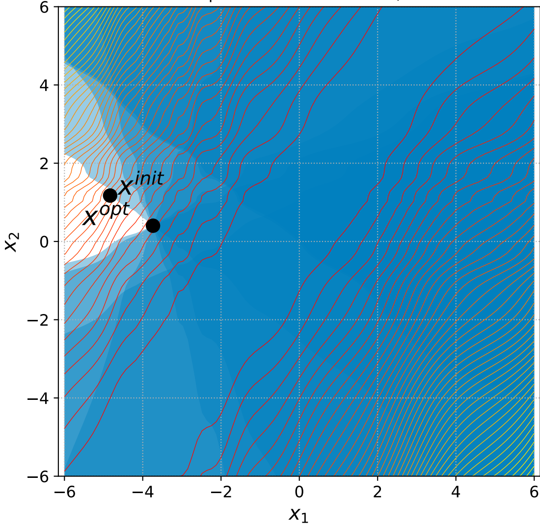
21 Rotated Ellipsoid with 6 constraints, instance=10
