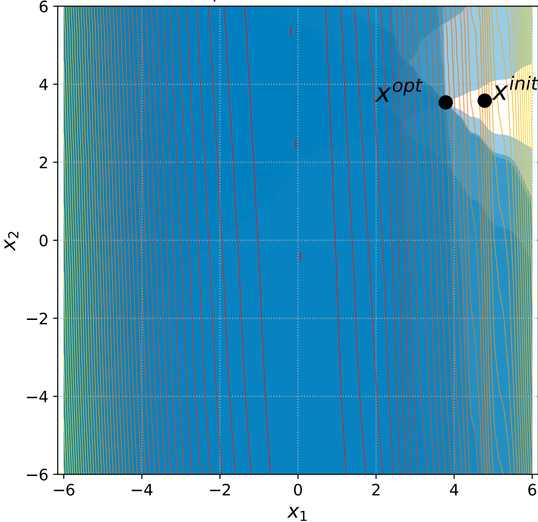
21 Rotated Ellipsoid with 6 constraints, instance=9
