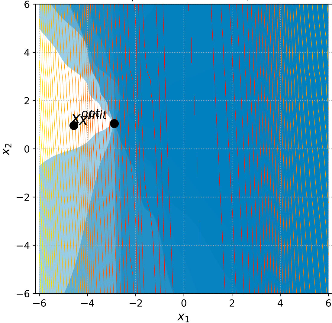
21 Rotated Ellipsoid with 6 constraints, instance=8
