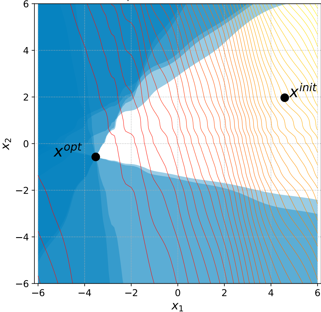
21 Rotated Ellipsoid with 6 constraints, instance=7
