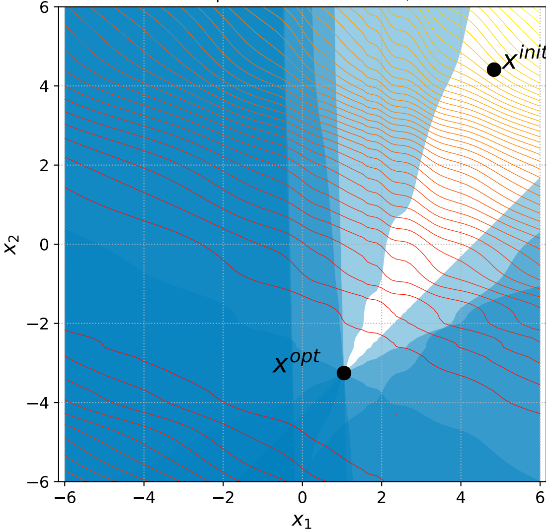
21 Rotated Ellipsoid with 6 constraints, instance=4
