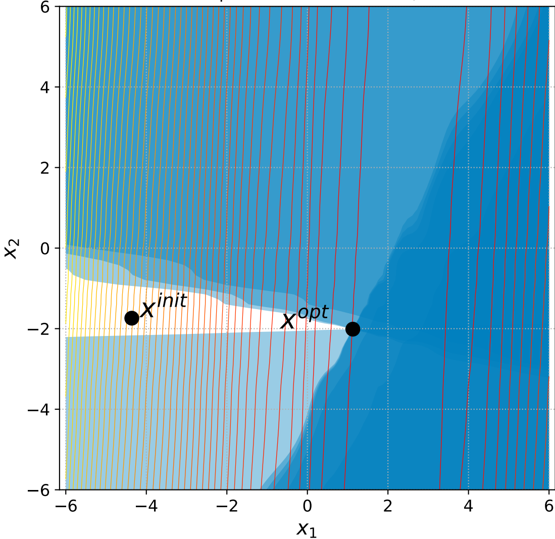
21 Rotated Ellipsoid with 6 constraints, instance=2
