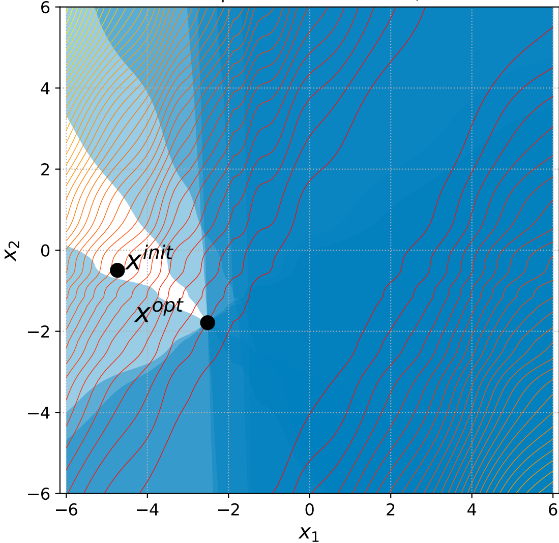
21 Rotated Ellipsoid with 6 constraints, instance=1
