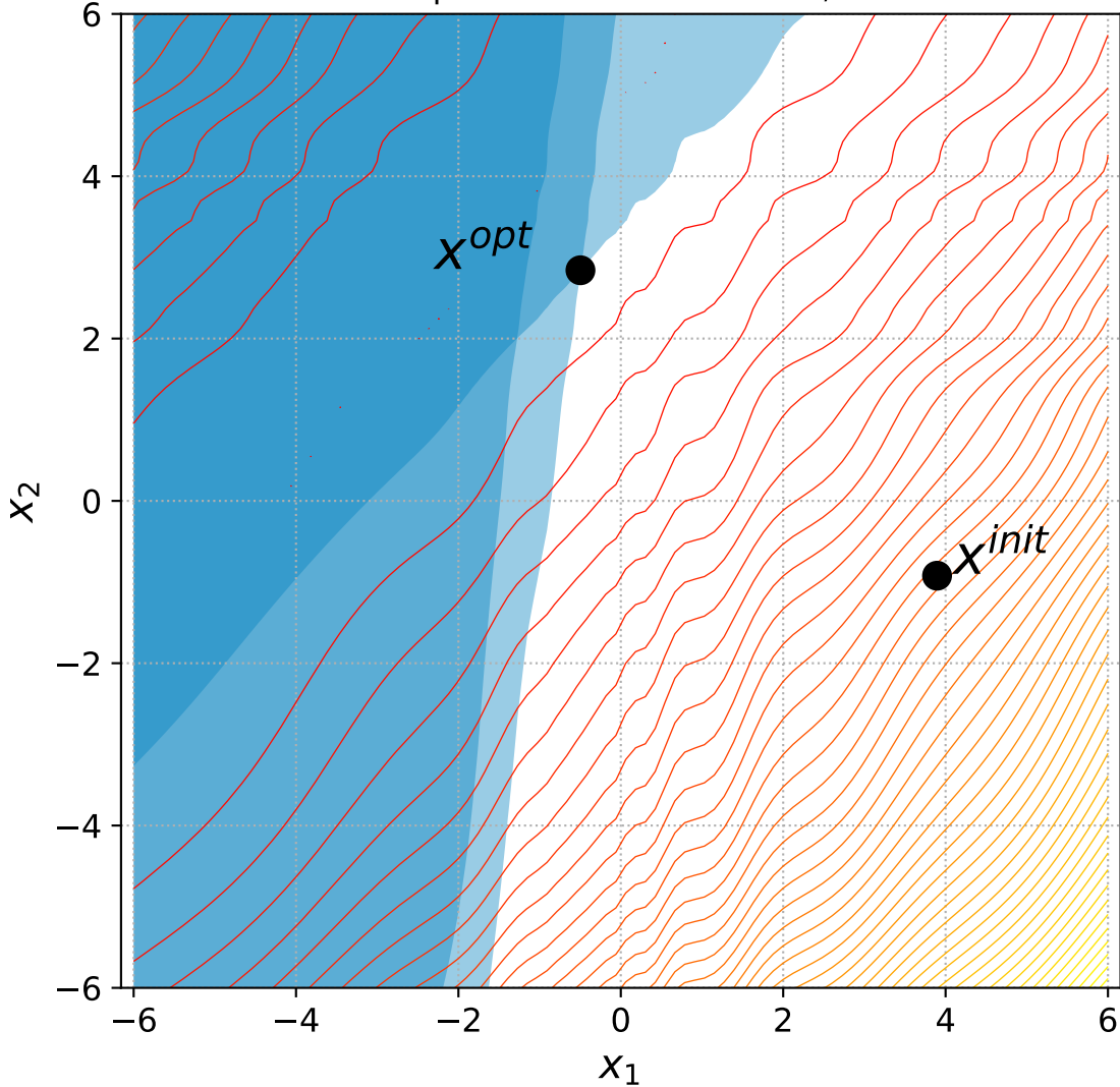
20 Rotated Ellipsoid with 2 constraints, instance=15
