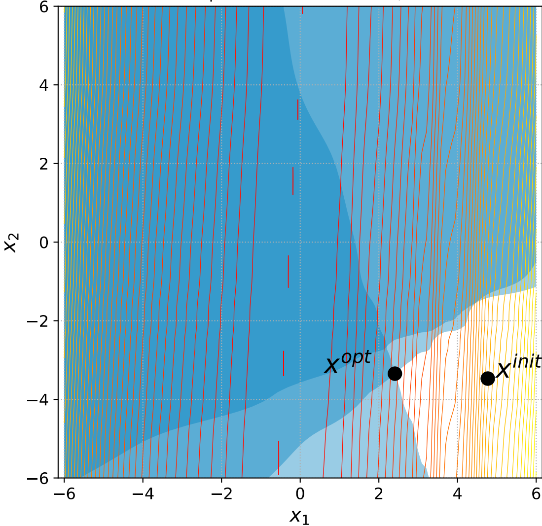
20 Rotated Ellipsoid with 2 constraints, instance=13
