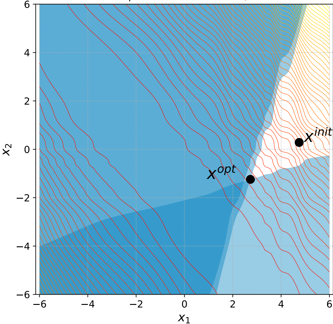
20 Rotated Ellipsoid with 2 constraints, instance=12
