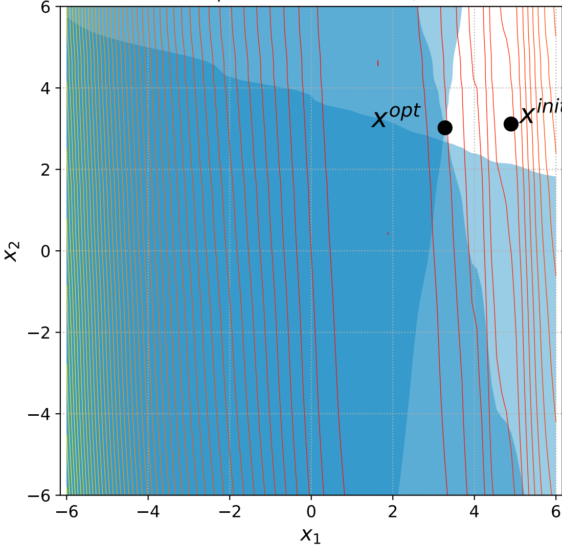
20 Rotated Ellipsoid with 2 constraints, instance=10
