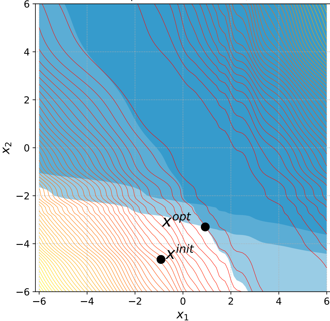
20 Rotated Ellipsoid with 2 constraints, instance=9
