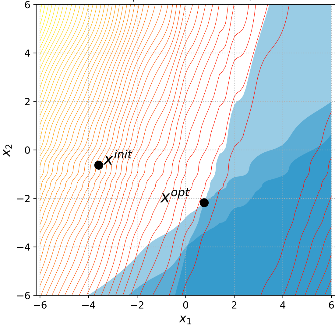
20 Rotated Ellipsoid with 2 constraints, instance=8
