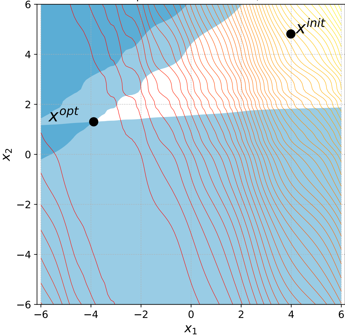
20 Rotated Ellipsoid with 2 constraints, instance=7
