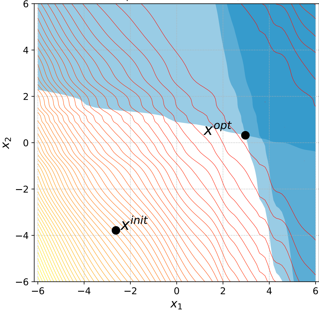
20 Rotated Ellipsoid with 2 constraints, instance=6
