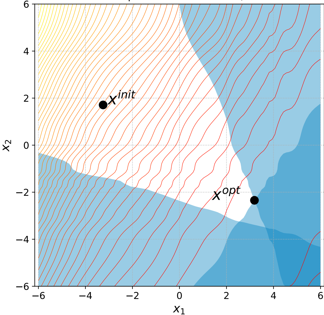
20 Rotated Ellipsoid with 2 constraints, instance=5
