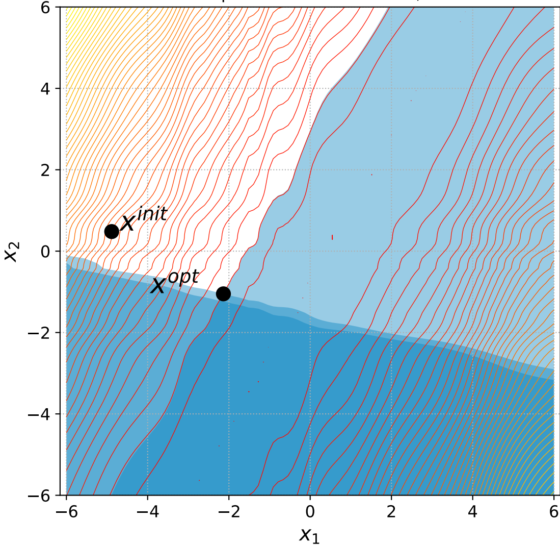
20 Rotated Ellipsoid with 2 constraints, instance=4
