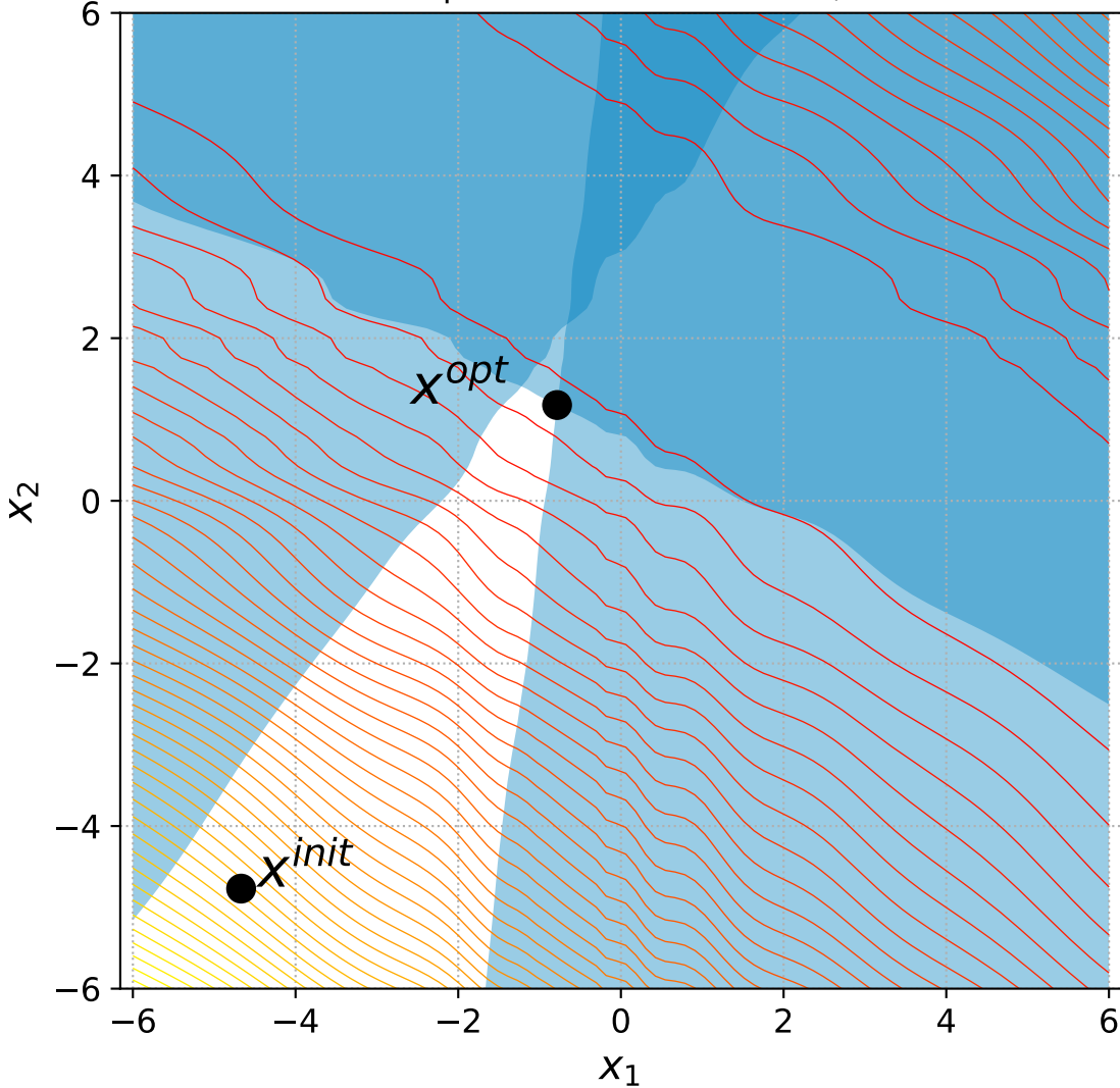
20 Rotated Ellipsoid with 2 constraints, instance=3
