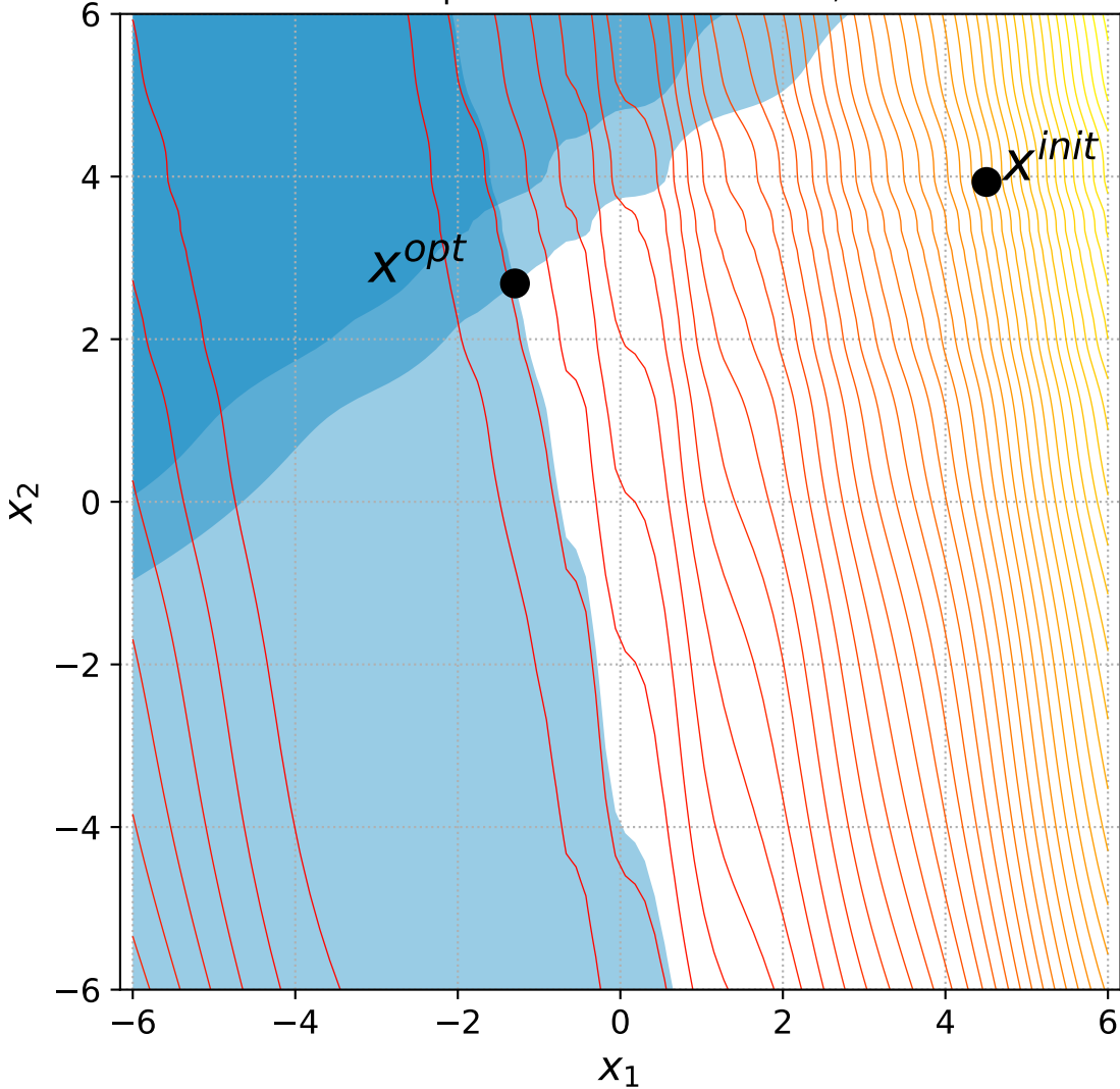
20 Rotated Ellipsoid with 2 constraints, instance=2
