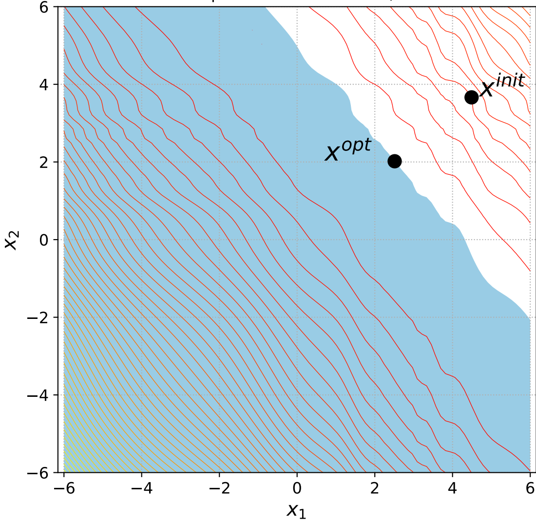
19 Rotated Ellipsoid with 1 constraint, instance=14
