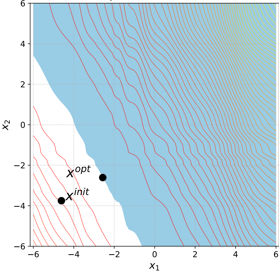
19 Rotated Ellipsoid with 1 constraint, instance=10
