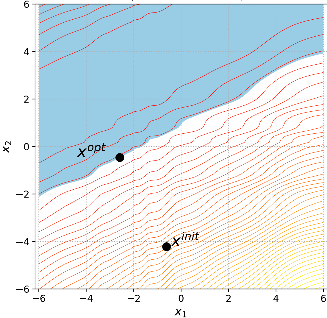
19 Rotated Ellipsoid with 1 constraint, instance=3
