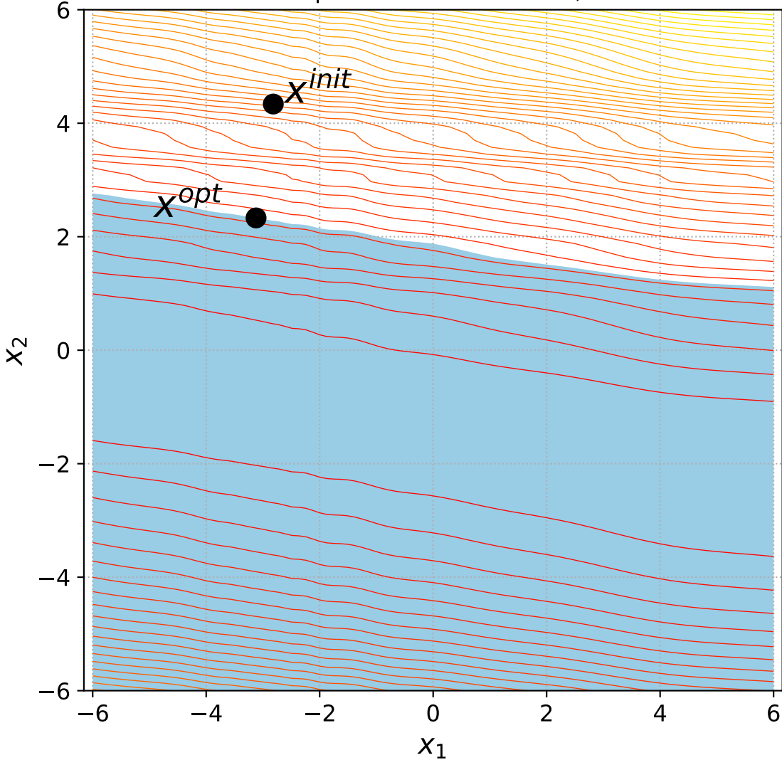
19 Rotated Ellipsoid with 1 constraint, instance=2
