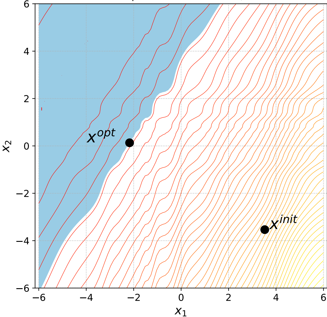
19 Rotated Ellipsoid with 1 constraint, instance=1
