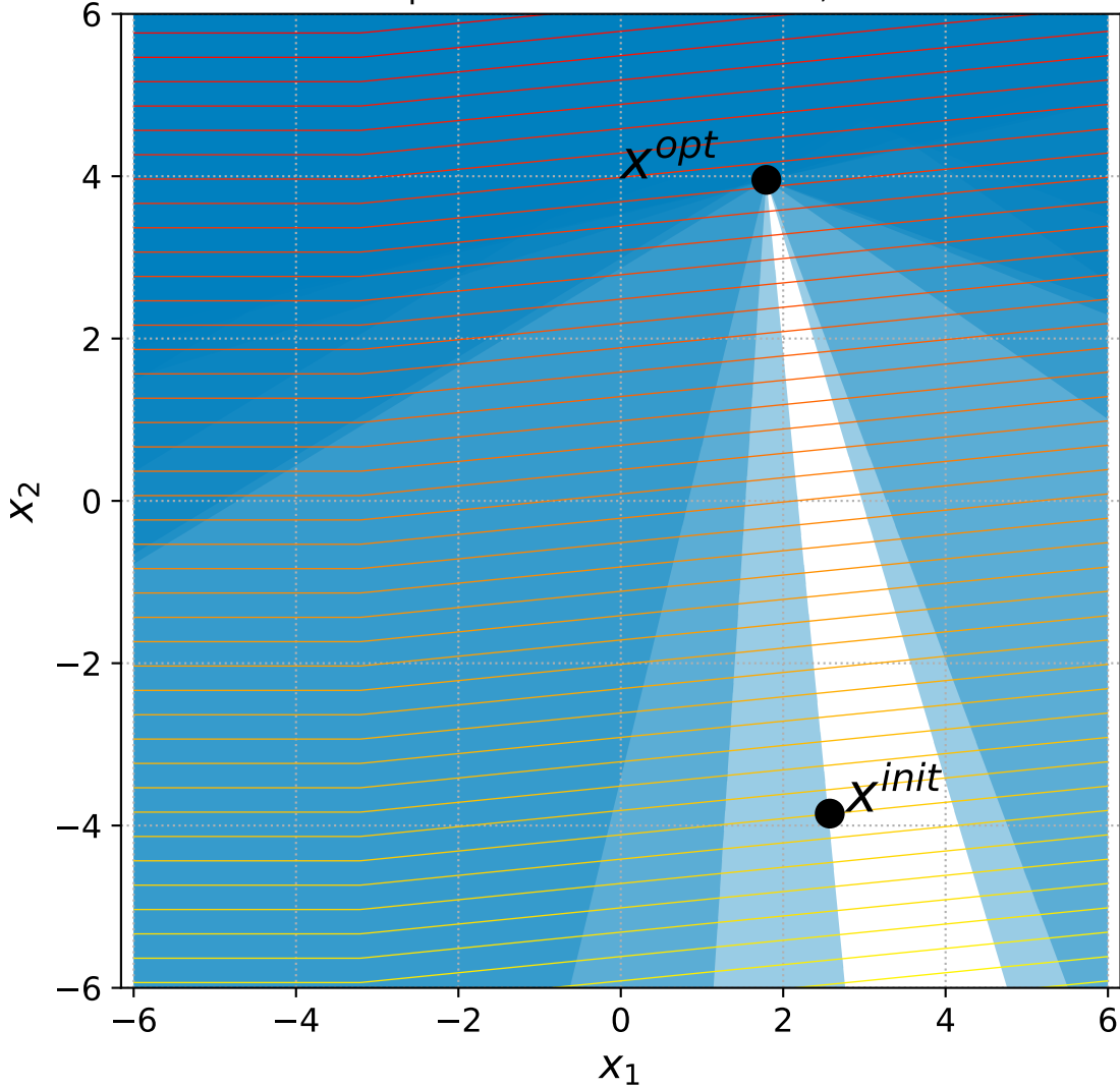
18 Linear Slope with 6+3n constraints, instance=14
