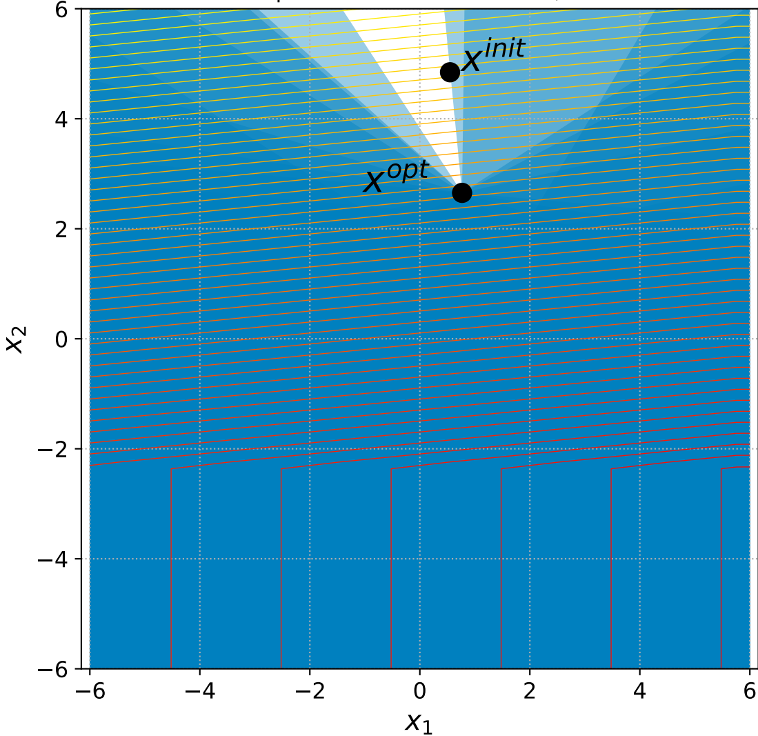
18 Linear Slope with 6+3n constraints, instance=12
