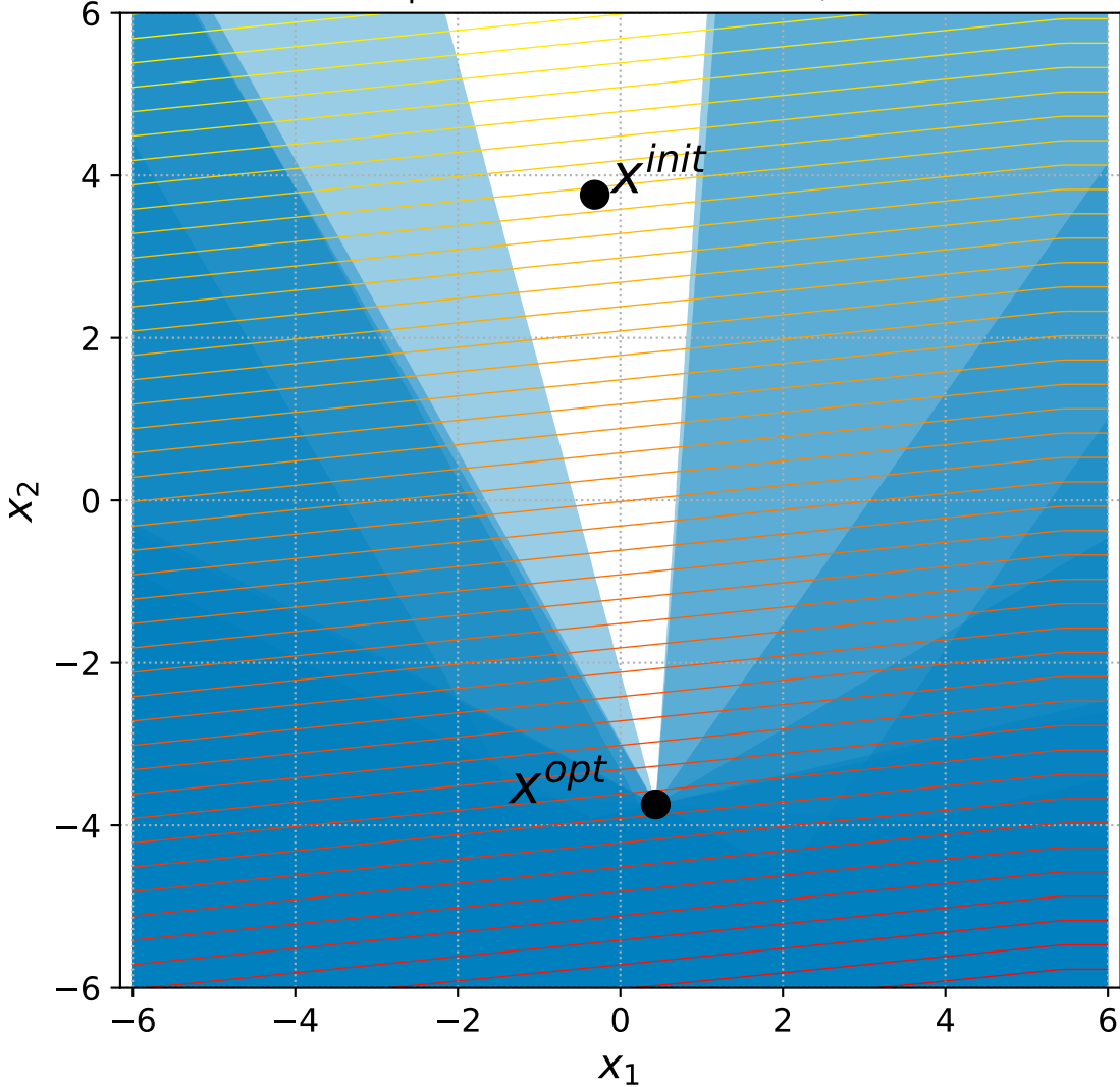
18 Linear Slope with 6+3n constraints, instance=11
