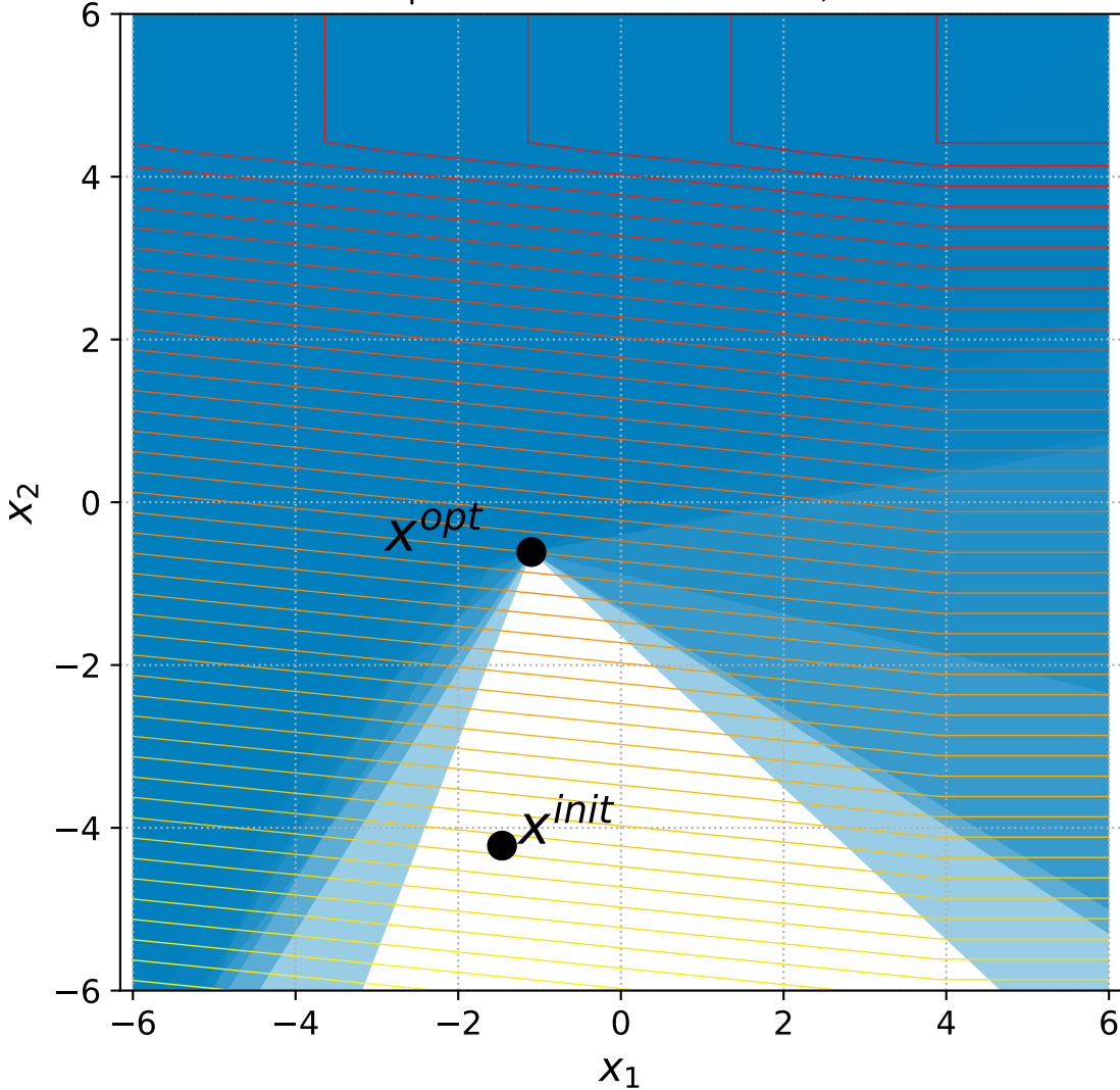
18 Linear Slope with 6+3n constraints, instance=10
