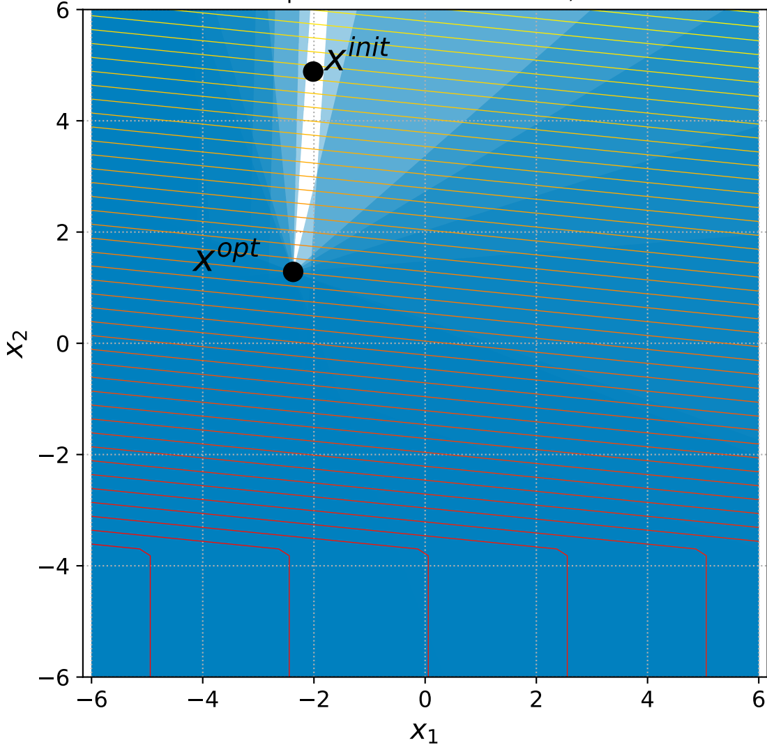
18 Linear Slope with 6+3n constraints, instance=9
