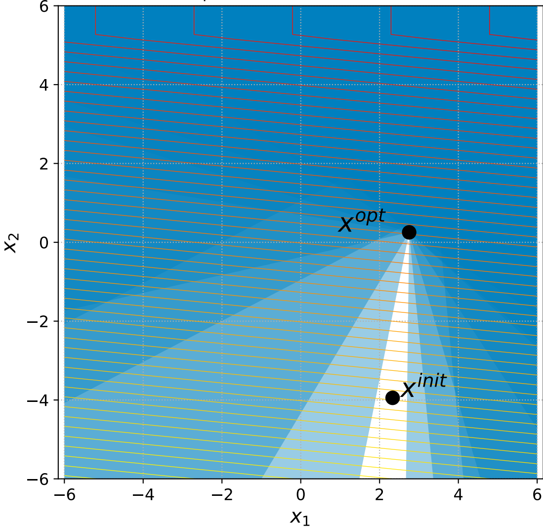
18 Linear Slope with 6+3n constraints, instance=7
