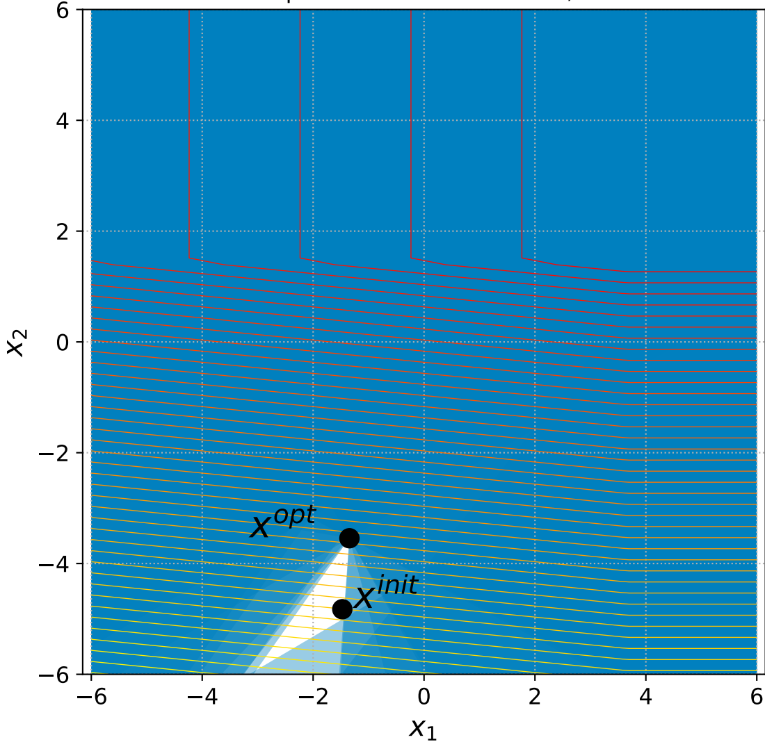
18 Linear Slope with 6+3n constraints, instance=6
