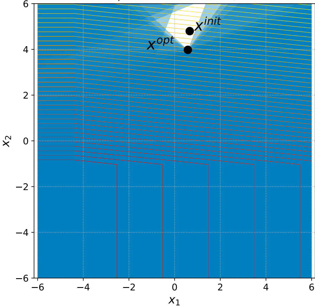
18 Linear Slope with 6+3n constraints, instance=5
