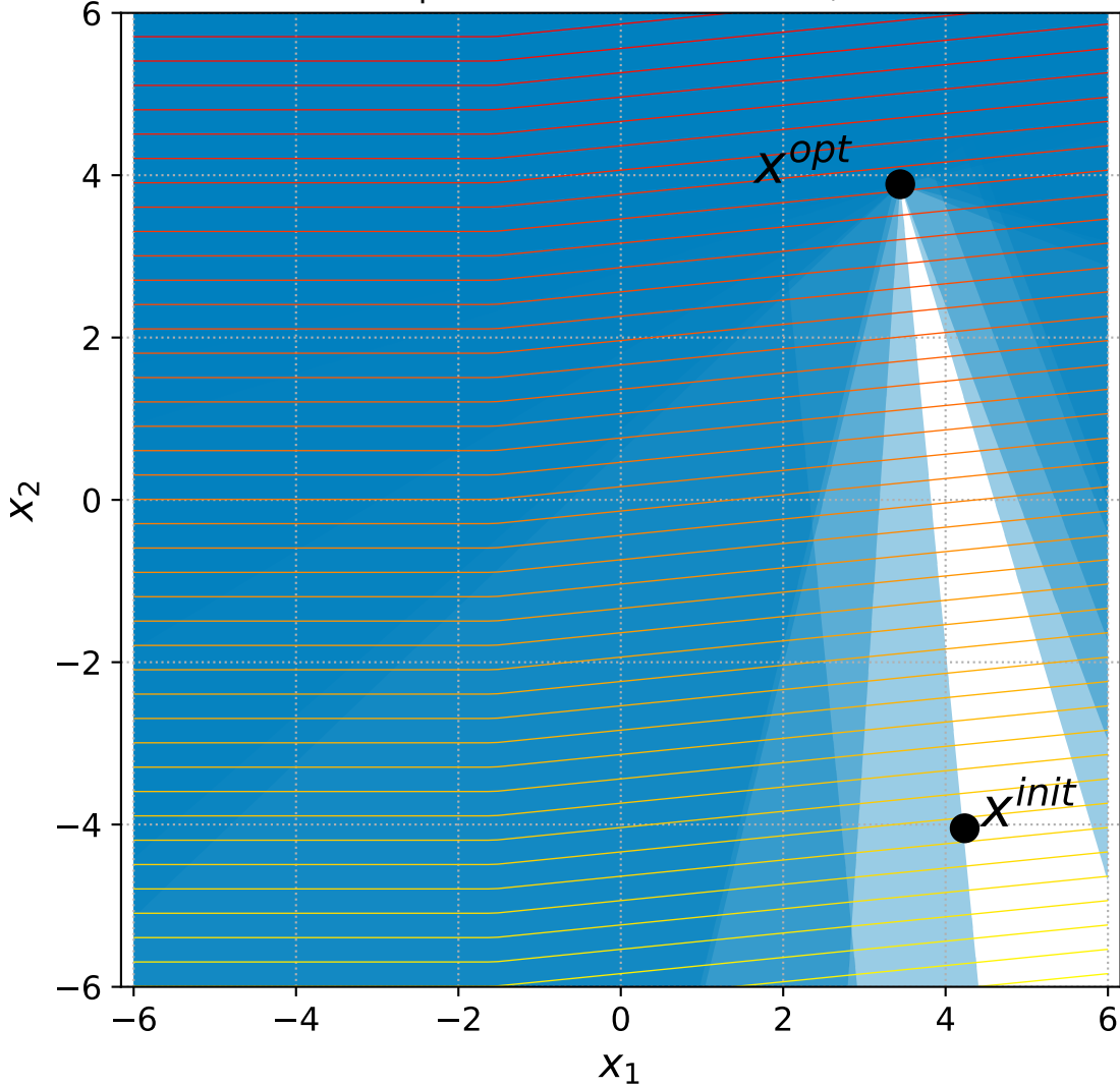
18 Linear Slope with 6+3n constraints, instance=4
