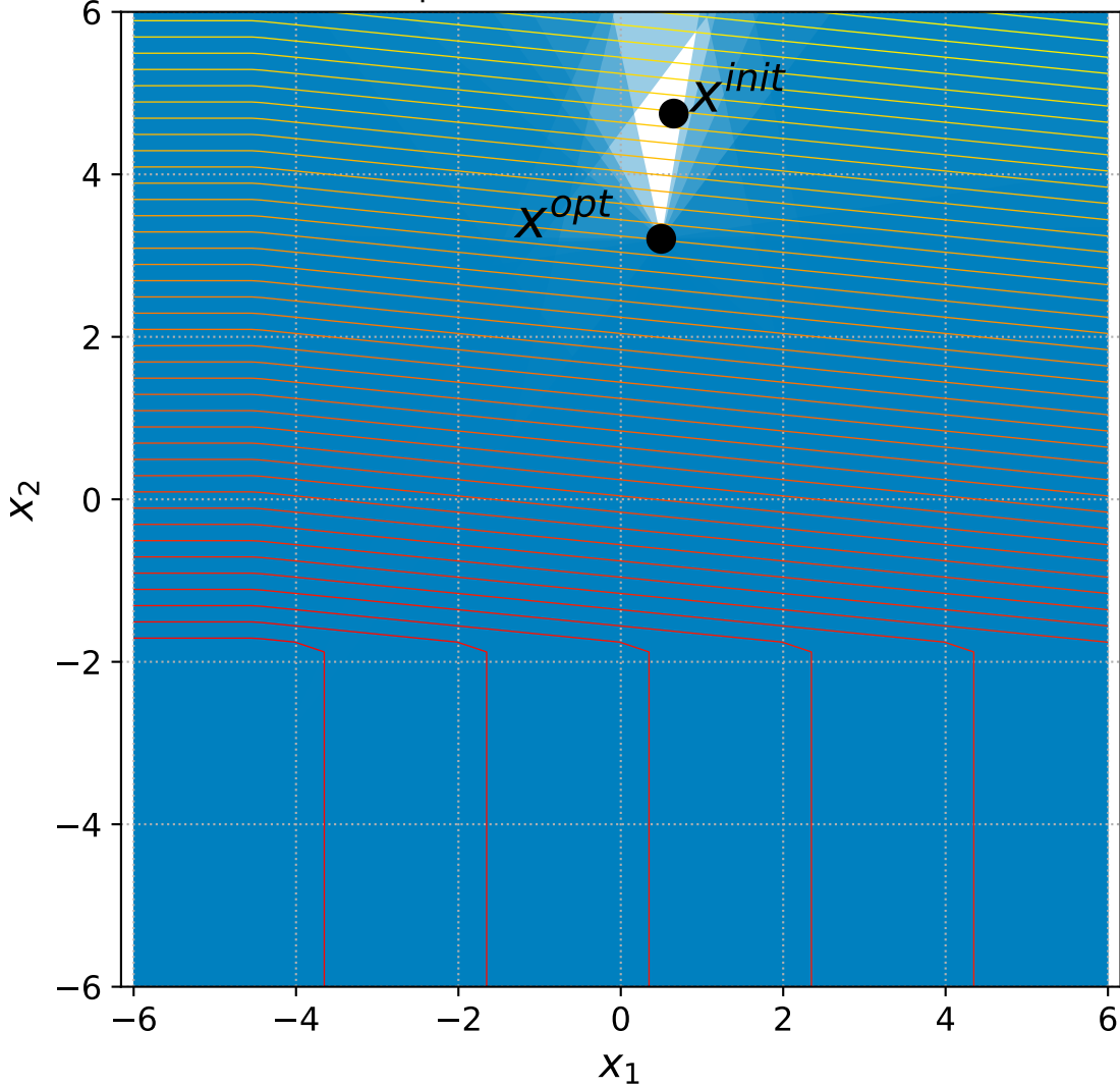
18 Linear Slope with 6+3n constraints, instance=3
