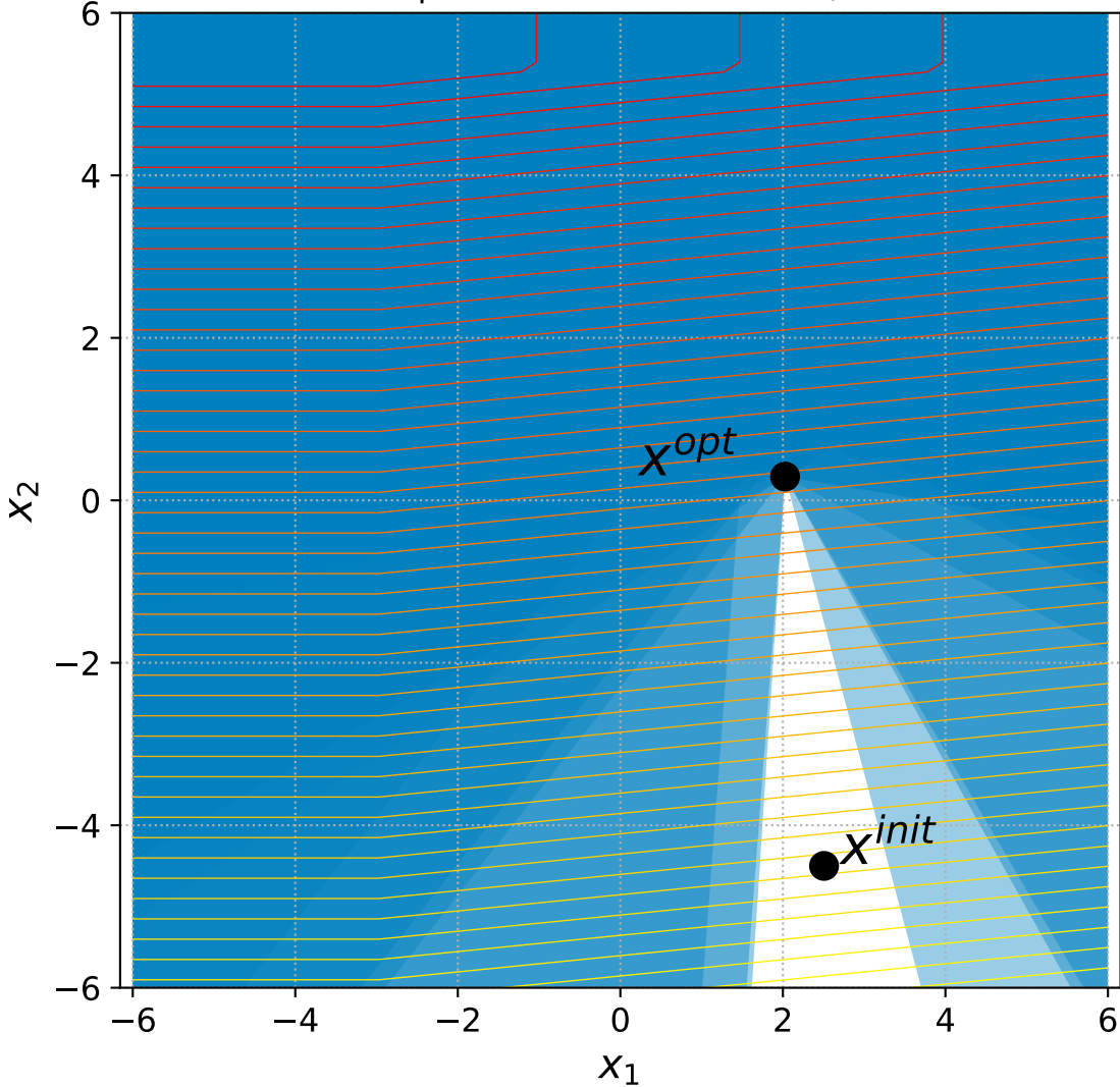
18 Linear Slope with 6+3n constraints, instance=1
