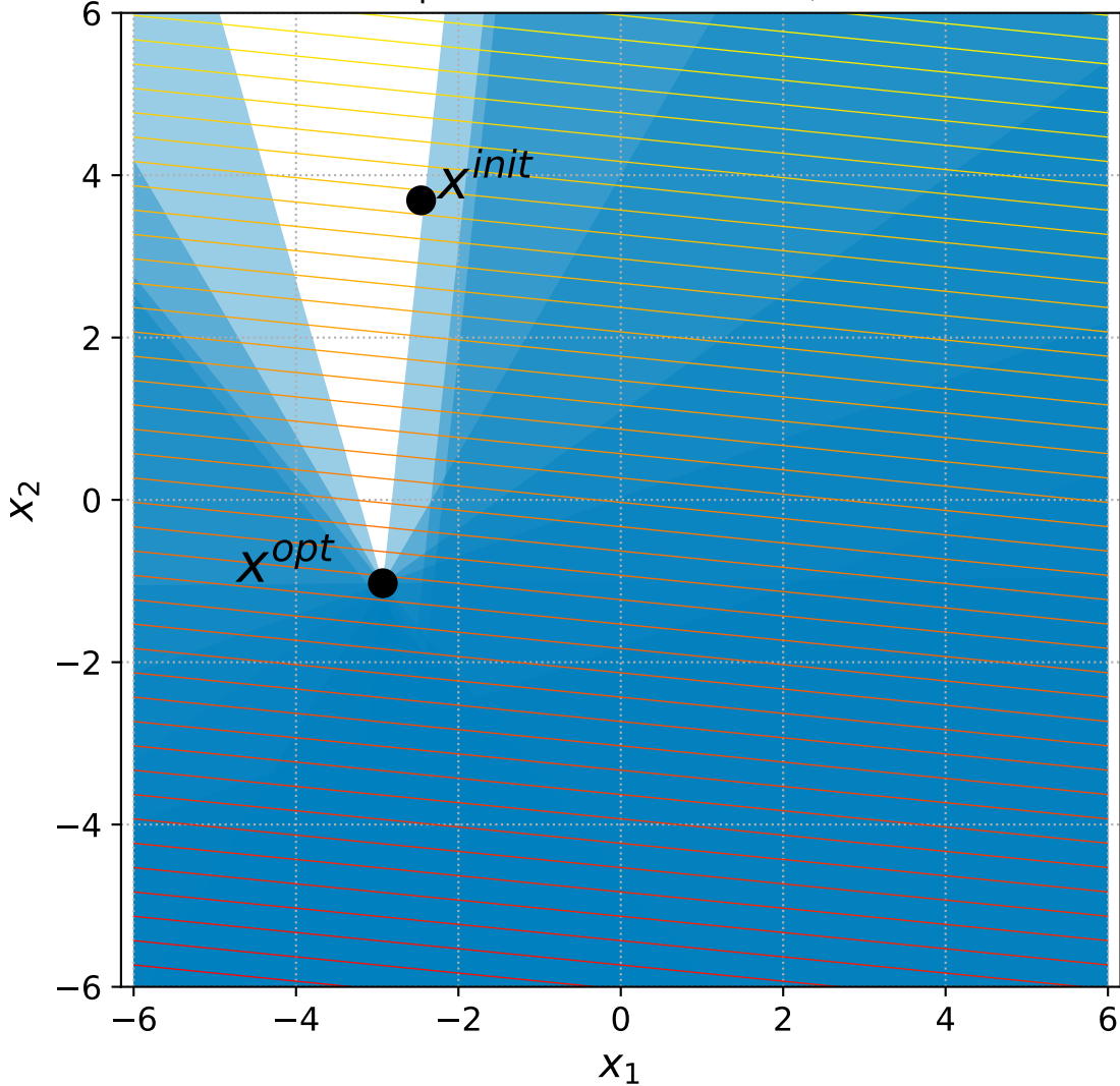
17 Linear Slope with 6+n constraints, instance=14
