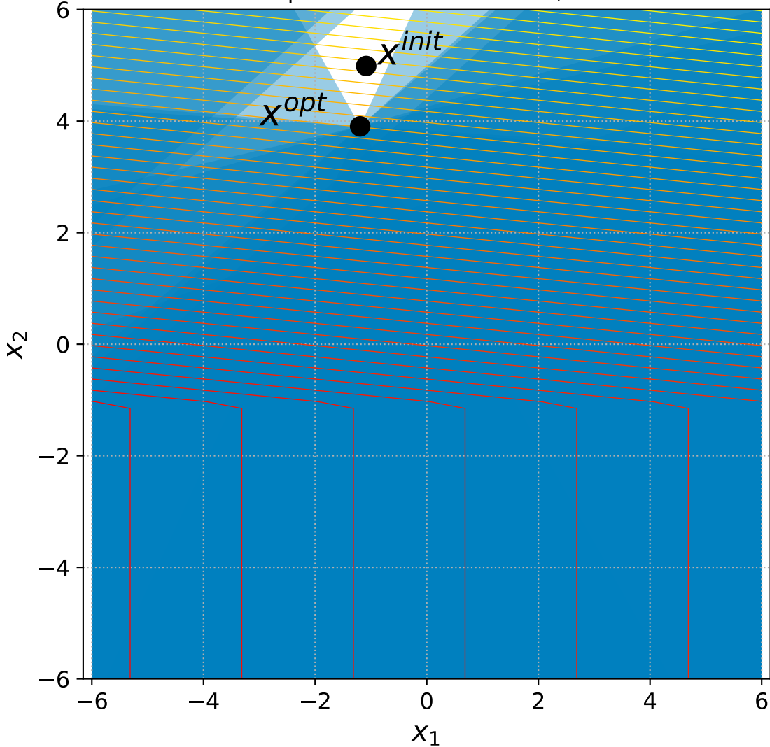
17 Linear Slope with 6+n constraints, instance=13
