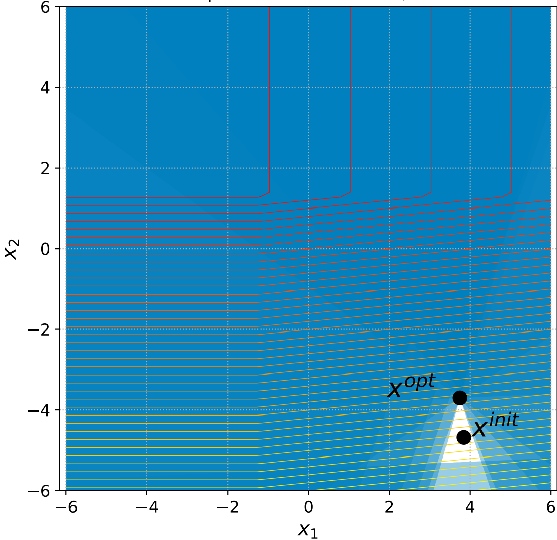
17 Linear Slope with 6+n constraints, instance=12
