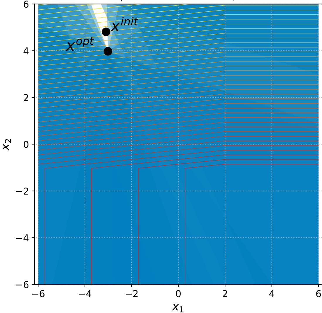
17 Linear Slope with 6+n constraints, instance=11
