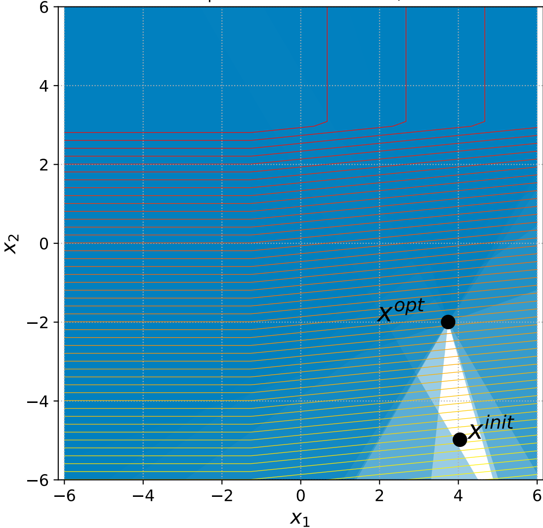
17 Linear Slope with 6+n constraints, instance=9
