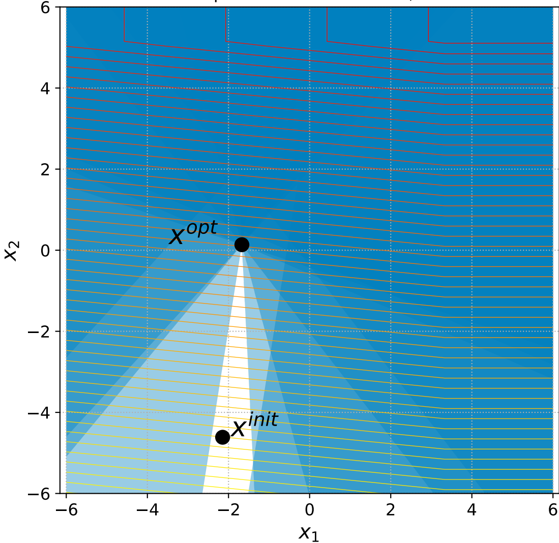
17 Linear Slope with 6+n constraints, instance=5
